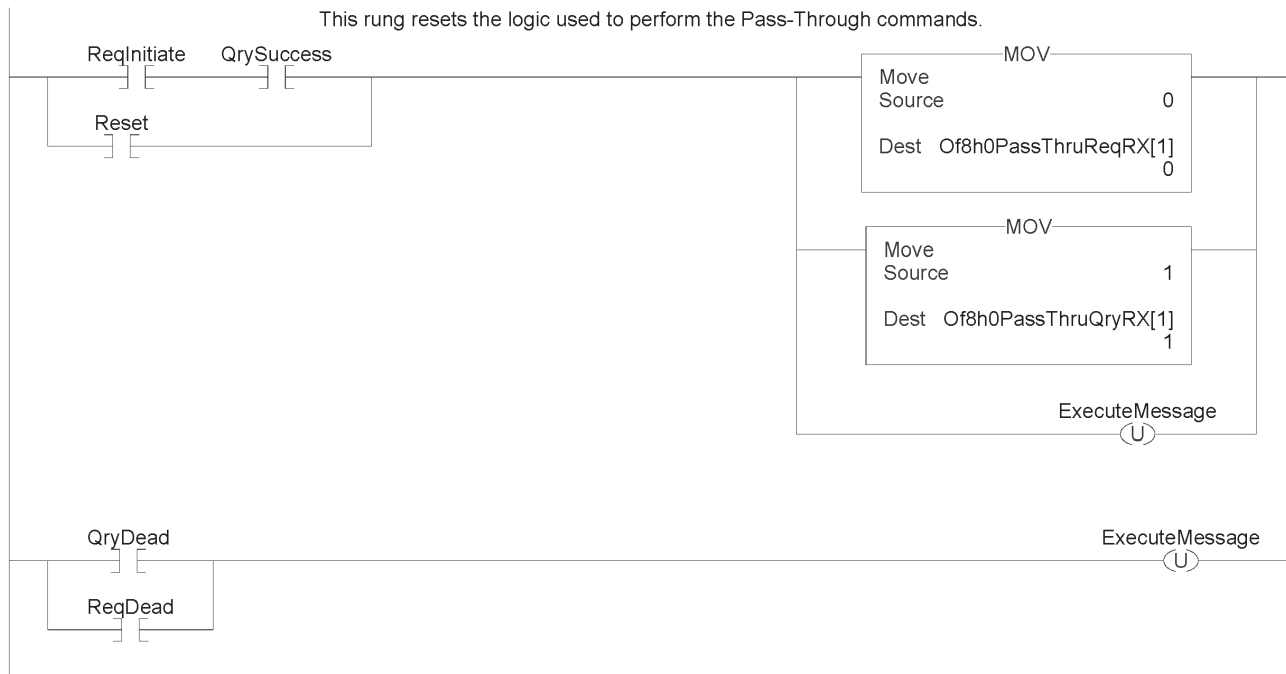
Figure 8.4e (OF8H HART Message Ladder)
