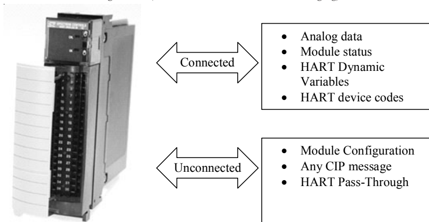
Figure 7.4 (Connected and Unconnected messaging)
