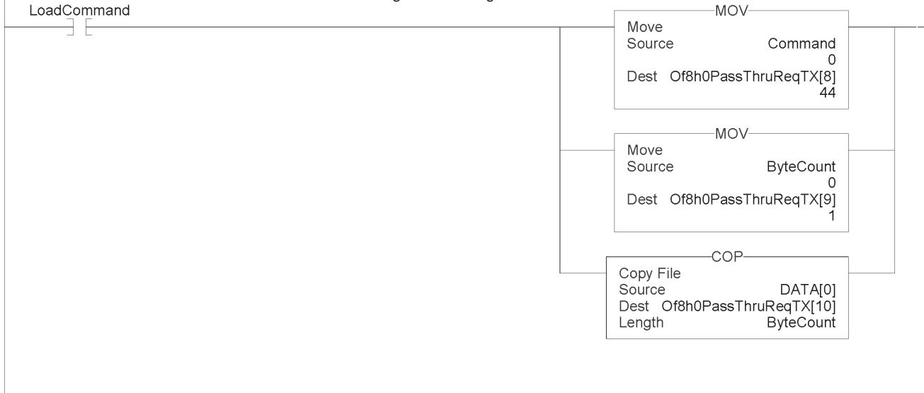
Figure 8.4b (OF8H HART Message Ladder)
