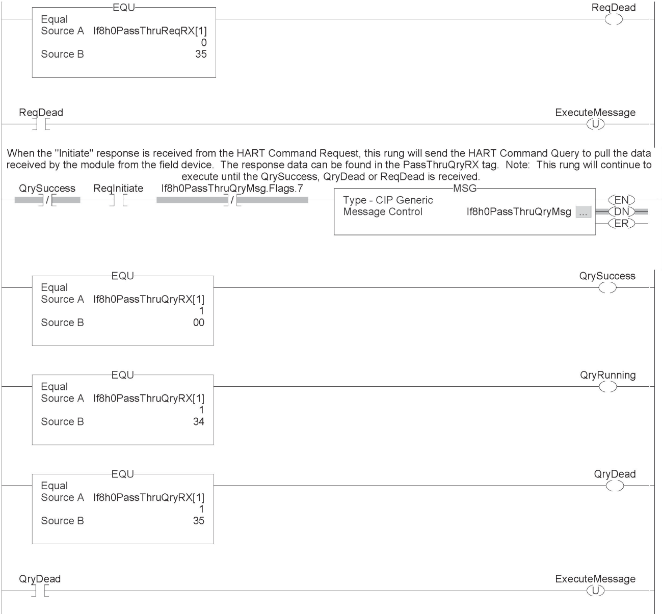
Figure 8.3d (IF8H HART Message Ladder)
