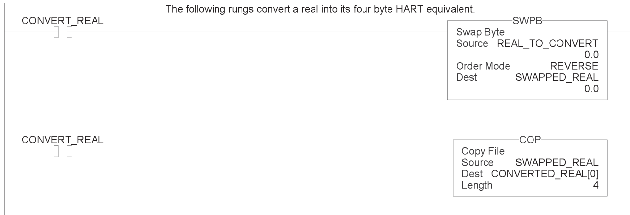
Figure 8.5 (Converting a FLOAT Value To Its 4 byte HART Equivalent)
