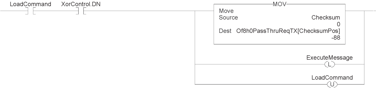
Figure 8.4c (OF8H HART Message Ladder)
