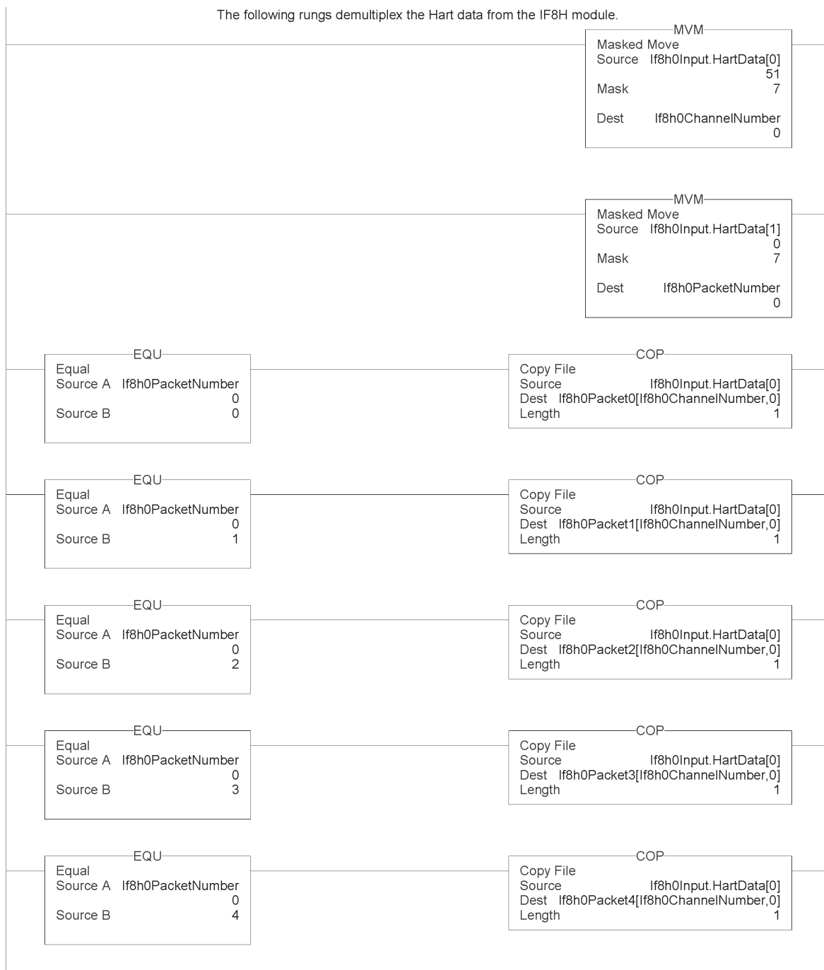
Figure 7.6 (Demultiplexing Ladder)
