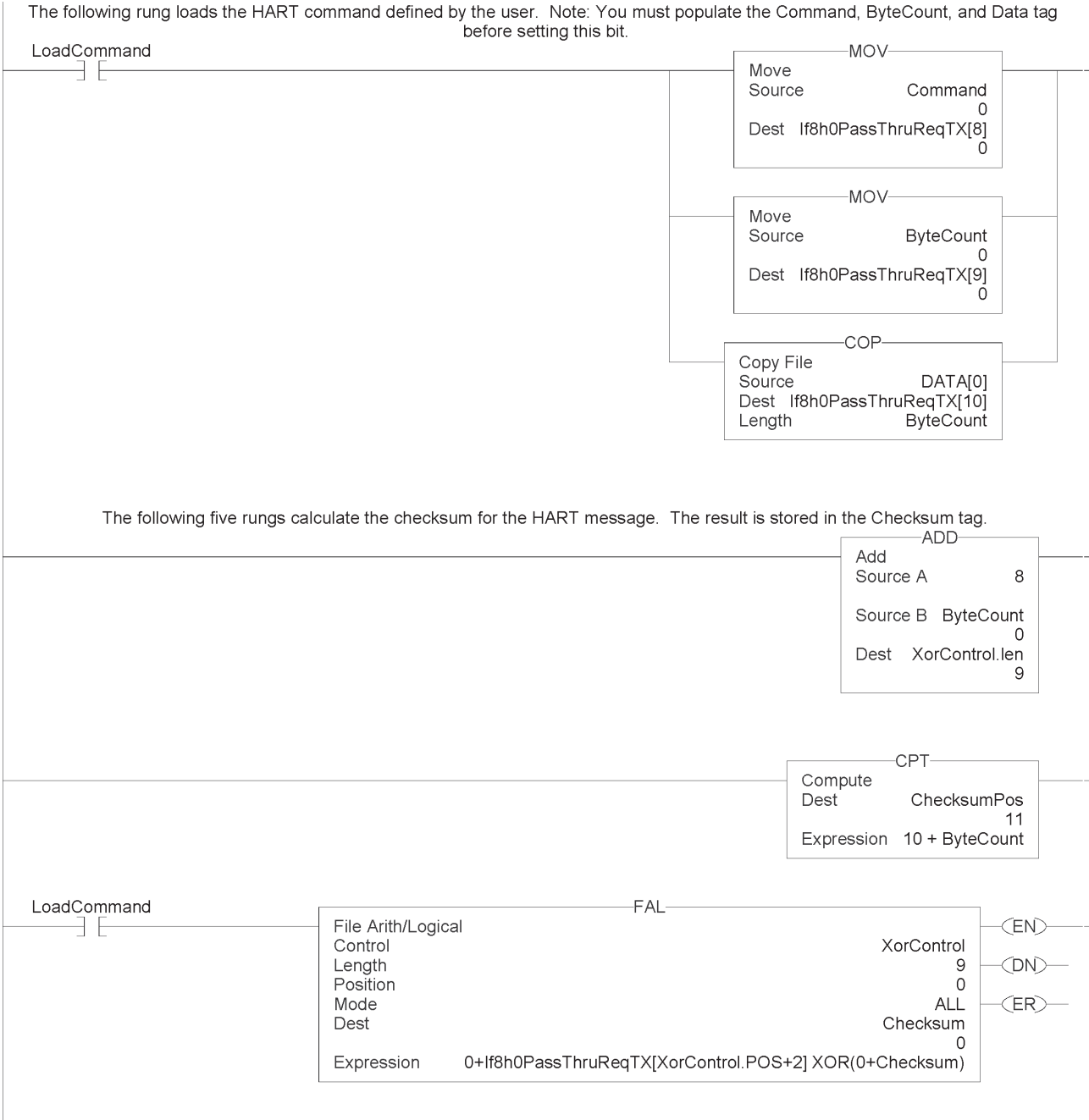
Figure 8.3b (IF8H HART Message Ladder)
